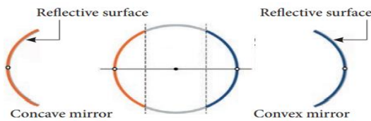
Figure 3.1 Spherical mirrors
