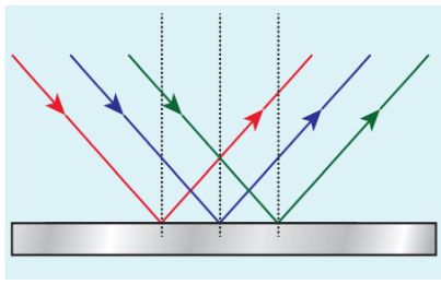
Regular reflection
