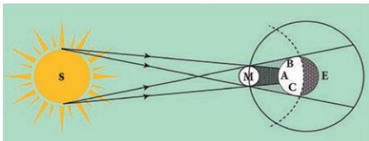
Solar eclipse
