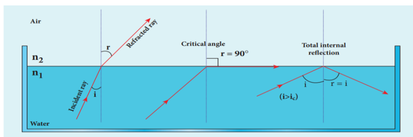
Figure 6.21 Critical angle and total internal reflection
